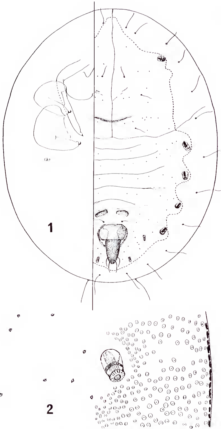
Figures 1, 2. Aleurodeus cocois , puparium (after Martin, 1987). 1, whole puparium, dorsal detail to right of line, boundary of submarginal wide-rimmed pore band shown as dashed line; 2, dorsal detail of abdominal segments III/III to show submarginal wide-rimmed pores, scattered subdorsal septate pores and large compound pore in lateral aspect.
